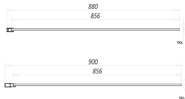
Dimensions (measurements in mm)
