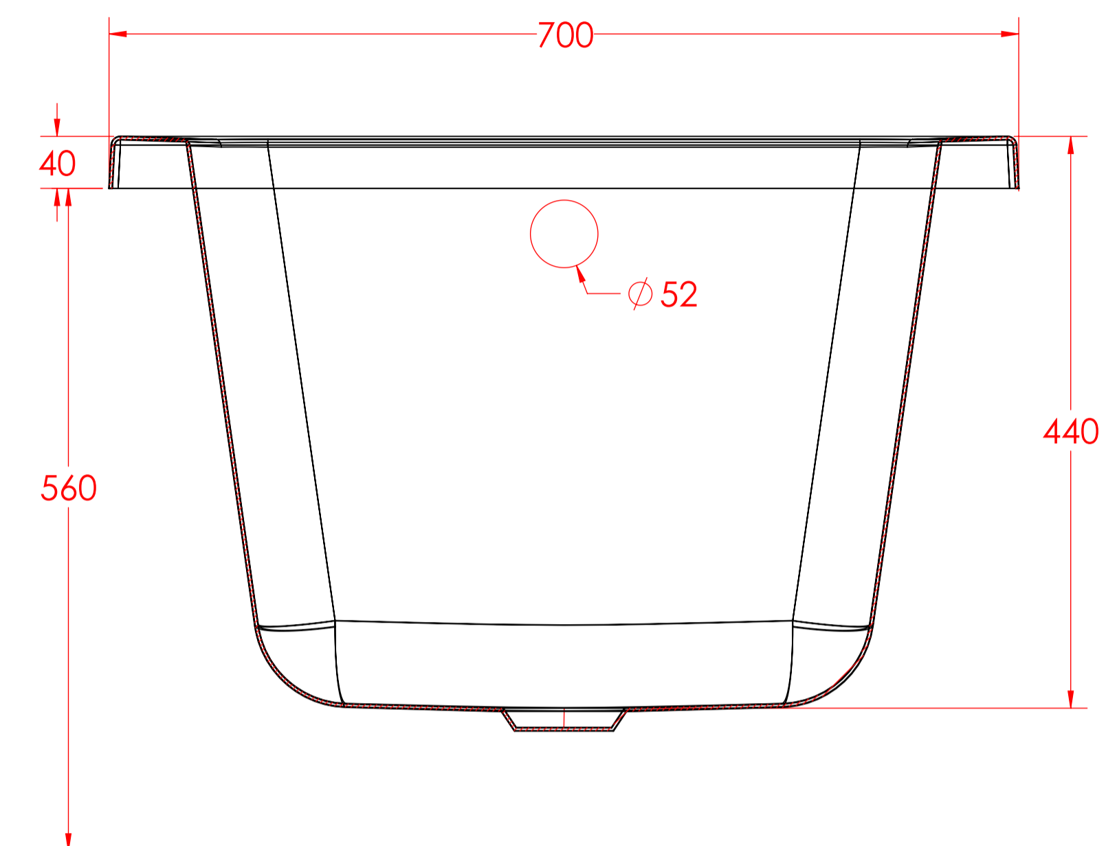
SECTION C-C SCALE 1 : 4
