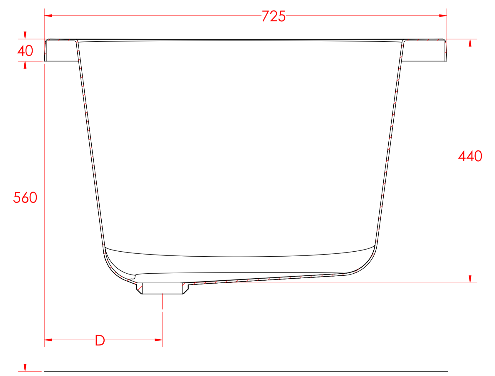
SECTION E-E SCALE 1 : 4
