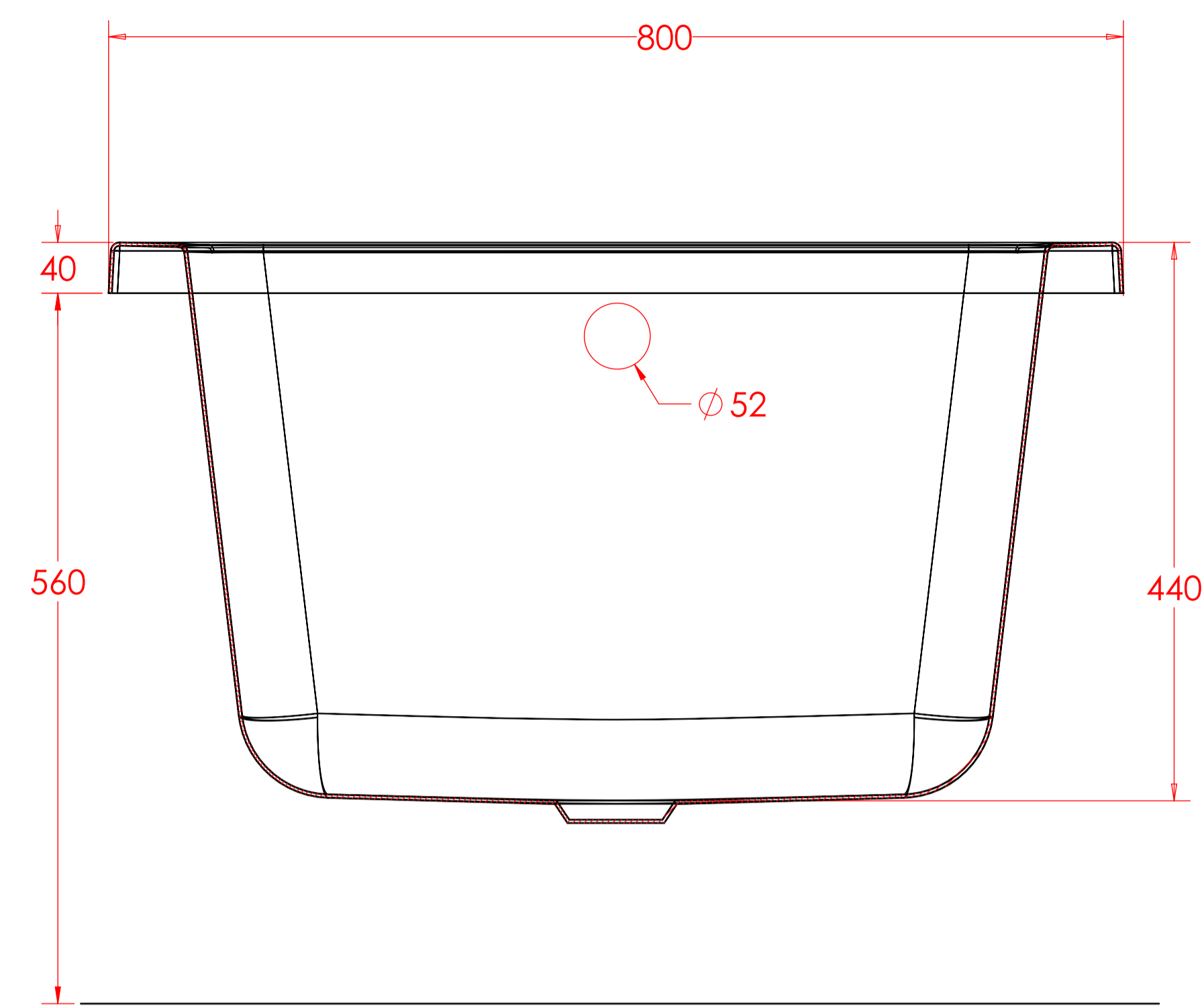
SECTION C-C SCALE 1 : 4
