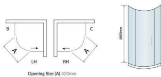
Opening Size (A) 420mm
