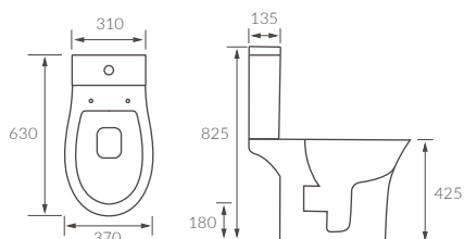
CLOSE COUPLED PAN AND CISTERN
