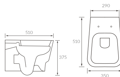
WALL HUNG PAN
