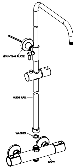
Step 4: Apply washer into the bottom of sliding rail, then fix the sliding rail onto the mixer body. Make markings for the position of the mounting plate, then take off the sliding rail.
