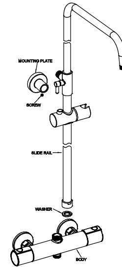
Step 6: Apply washer into the bottom of sliding rail then fix the sliding rail onto the mixer body. Then fix sliding rail onto mounting plate, tighten with screws.
