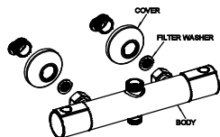
Step 3: Attach the covers against wall, place filters into the inlets. Then fix mixer onto the wall with spanner, checking for leakage.
