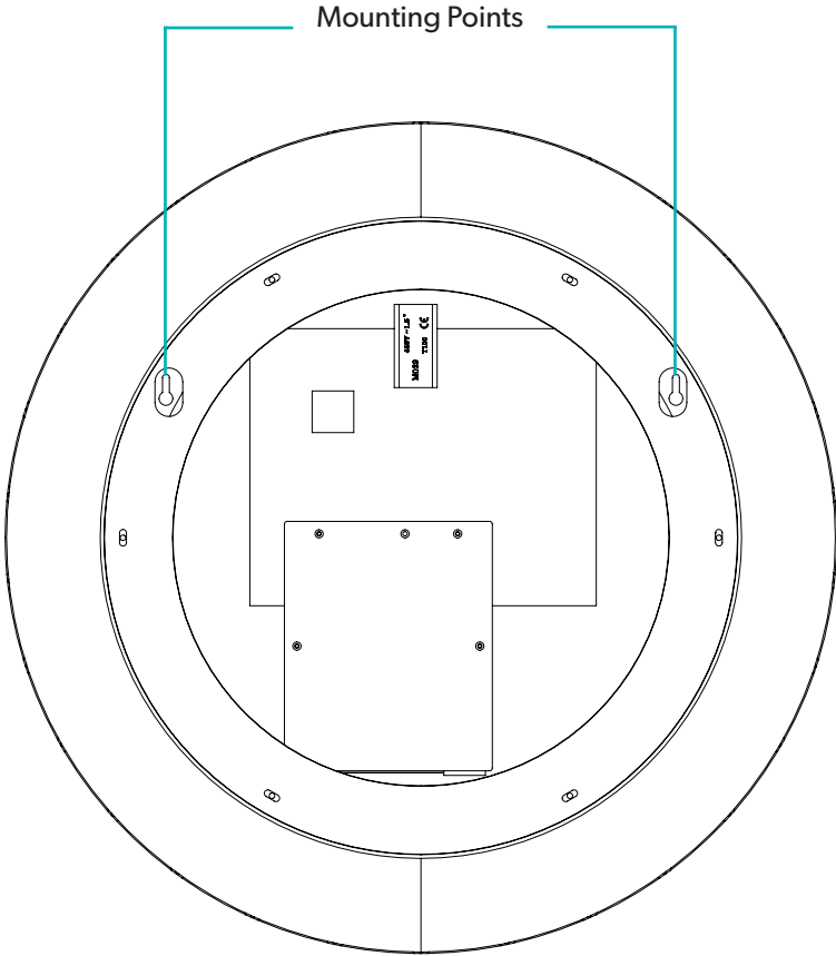
Fig 2. - Mounting points
